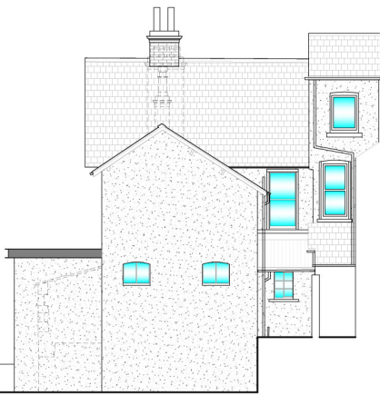
AS PROPOSED EAST ELEVATION (Scale 1:50)
