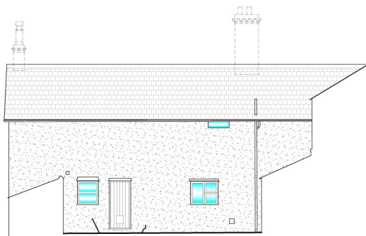
AS PROPOSED EAST ELEVATION (Scale 1:50)
